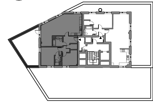
SIXTH FLOOR PLAN SCALE 1:500
